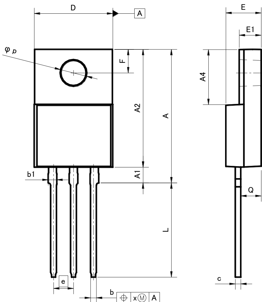
TO-220FM
