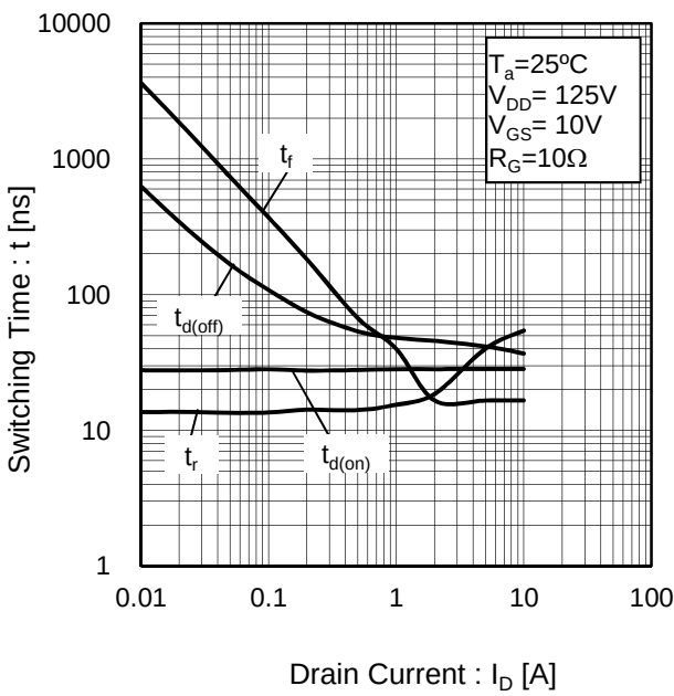
Fig.18 Switching Characteristics
