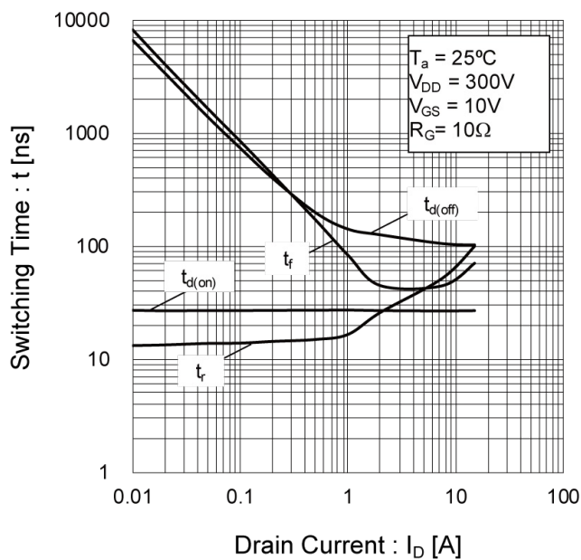
Fig.18 Switching Characteristics
