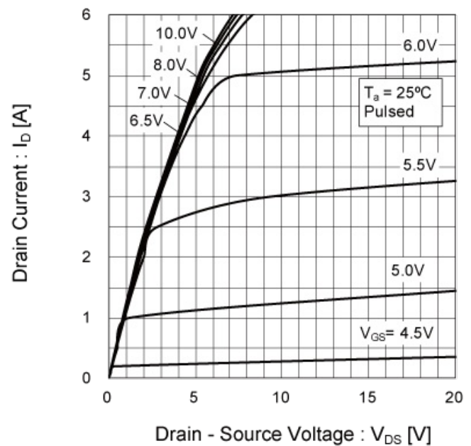
Fig.8 Output Characteristics(II)
