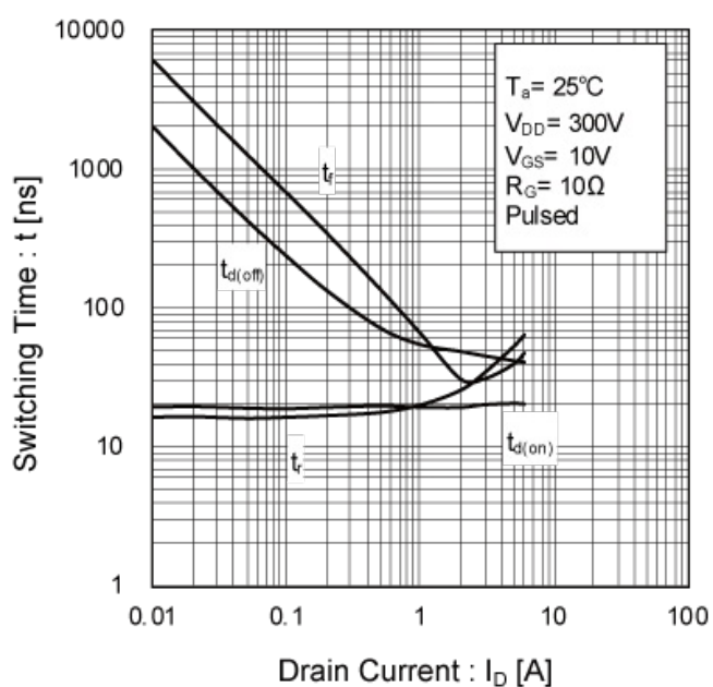
Fig.15 Switching Times
