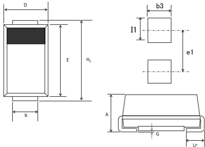
DO-214AC(SMA), (FMDS)
