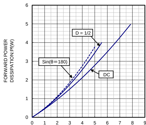
I_0 - P_f CHARACTERISTICS
