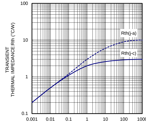
R_th-t CHARACTERISTICS
