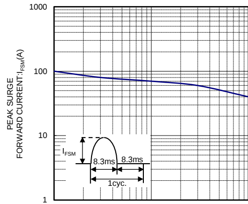
I_FSM-CYCLE CHARACTERISTICS
