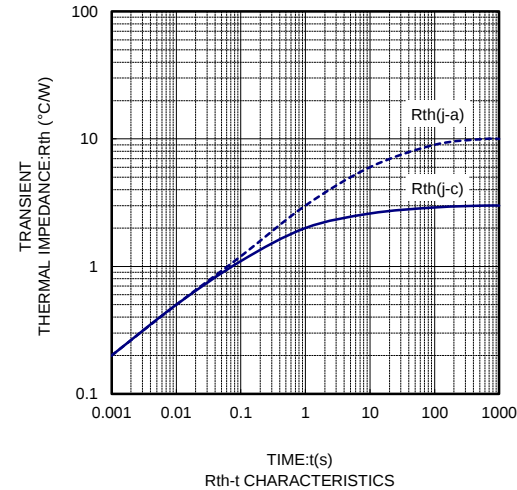
R_th-t CHARACTERISTICS
