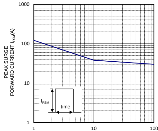
I_FSM-t CHARACTERISTICS
