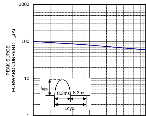
I_FSM-CYCLE CHARACTERISTICS
