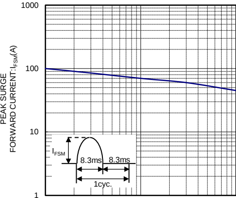
NUMBER OF CYCLES IFSM-CYCLE CHARACTERISTICS
