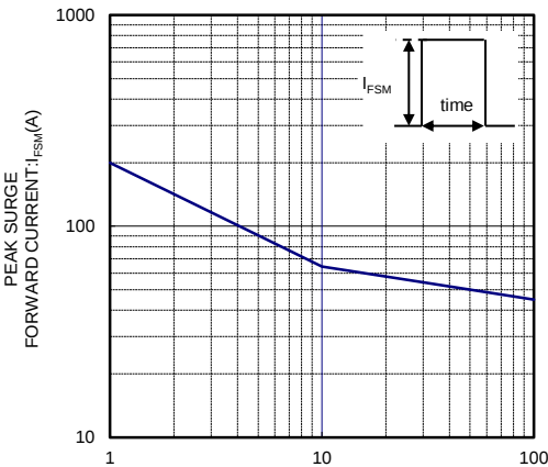
I_FSM-t CHARACTERISTICS
