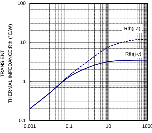
R_th-t CHARACTERISTICS
