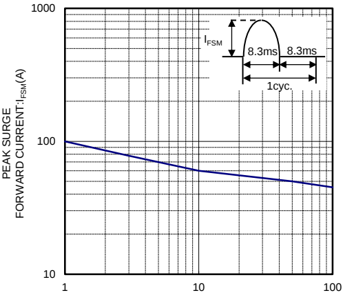
I_FSM-CYCLE CHARACTERISTICS
