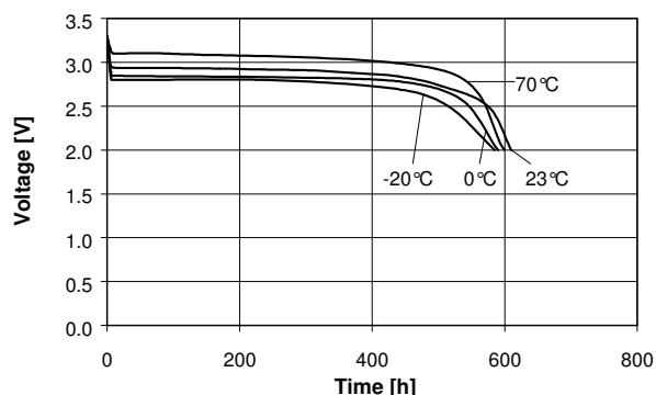
Temperature performance Load 25.5kΩ
