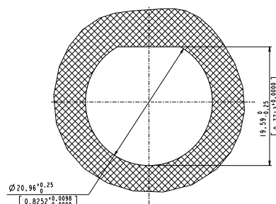
Panel Drilling
