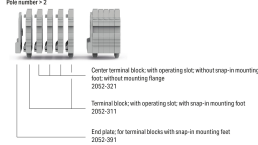
Example of a 5-pole terminal strip, with operating slots, with snap-in mounting foot
