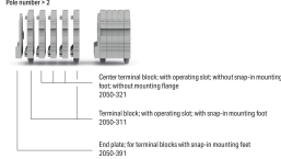
Example of a 5-pole terminal strip, with operating slots, with snap-in mounting feet
