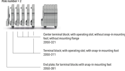
Example of a 5-pole terminal strip, with operating slots, with snap-in mounting foot
