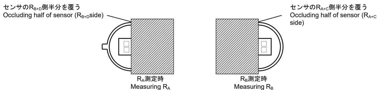
図6 出力電圧測定時のセンサ目隠し位置 Fig.6 Position of occluding sensor when measuring Responsivity
