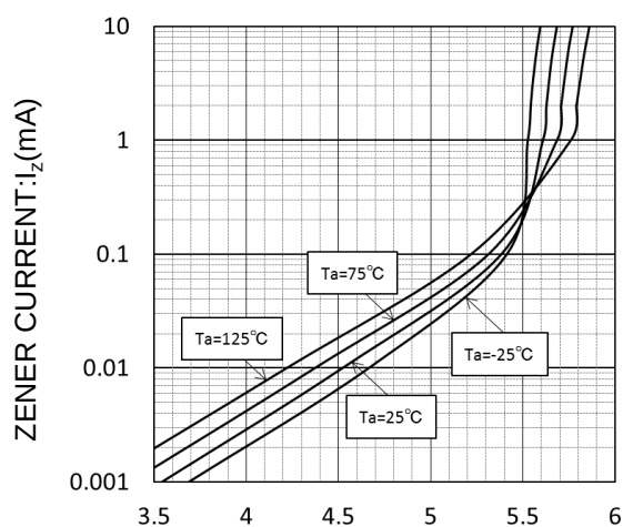
ZENER VOLTAGE: V_Z (V) V_Z - I_Z CHARACTERISTICS
