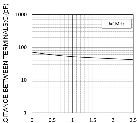
REVERSE VOLTAGE: V_R (V) V_R - C_t CHARACTERISTICS
