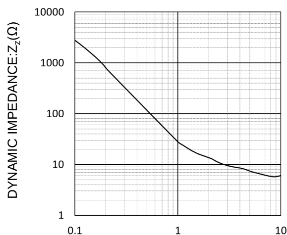
ZENER CURRENT: I_Z (mA) I_Z - Z_z CHARACTERISTICS
