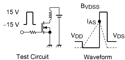
Fig. 8.16 Test Circuit/Waveform
