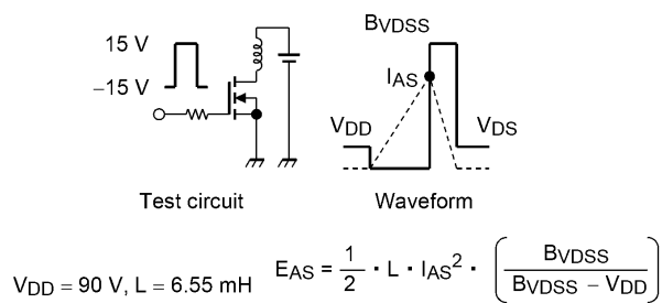
Fig. 8.16 Test Circuit/Waveform
