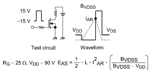
Fig. 8.16 Test Circuit/Waveform
