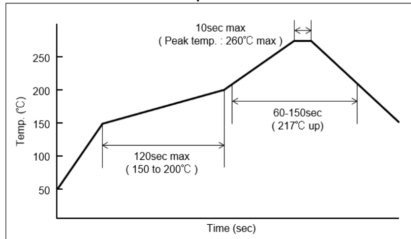
&lt; Figure 1. &gt; Our Recommended Reflow Profile
