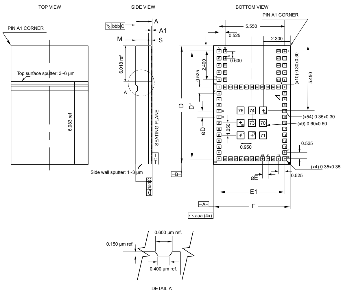
Figure 11. LGA77 - Outline
