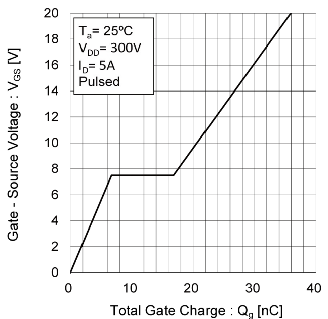
Fig.16 Gate charge
