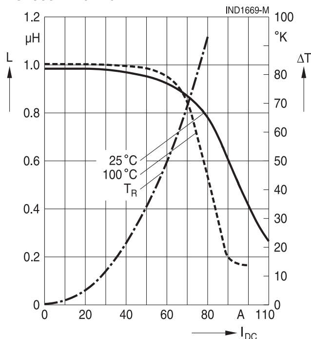
B82559A2102A024
