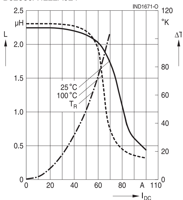
B82559A4222A024
