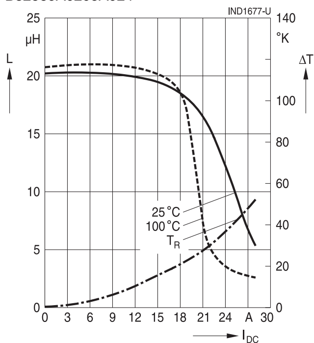
B82559A0203A024
