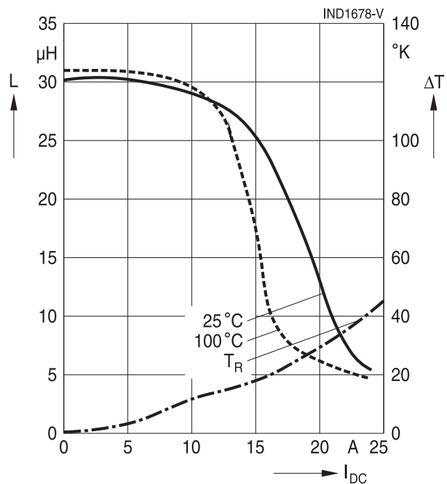
B82559A0303A024
