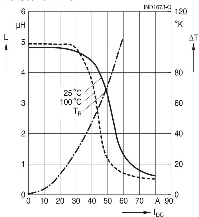
B82559A6472A024
