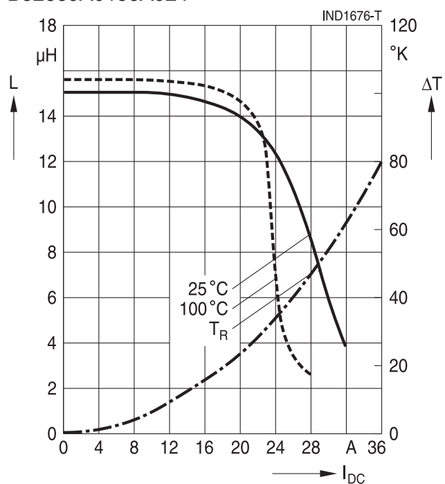
B82559A0153A024
