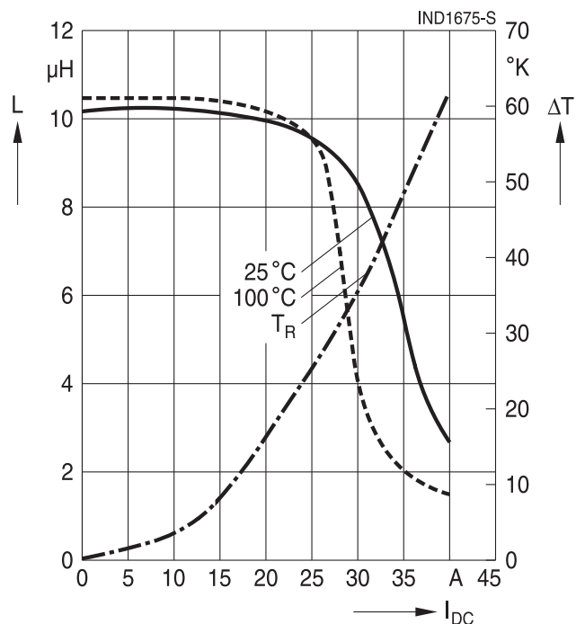
B82559A9103A024
