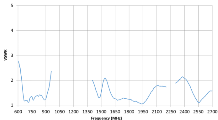
VSWR (600-2700 MHz)
