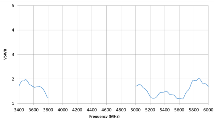
VSWR (3400-6000 MHz)
