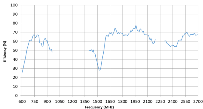
Efficiency (600-2700 MHz)
