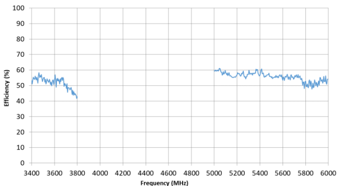
Efficiency (3400-6000 MHz)
