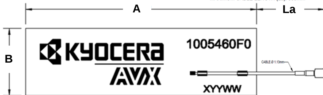
Top View
