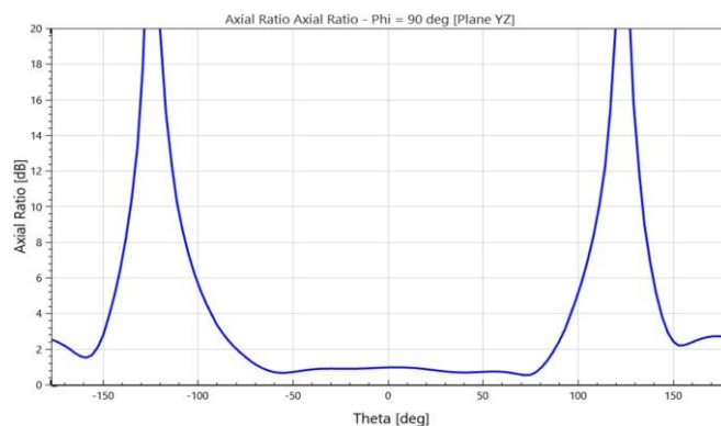
Axial Ratio (1585 MHz)
