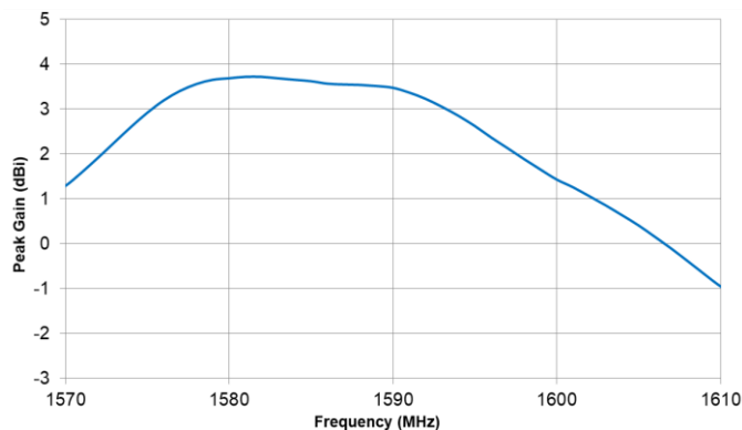
Peak Gain
