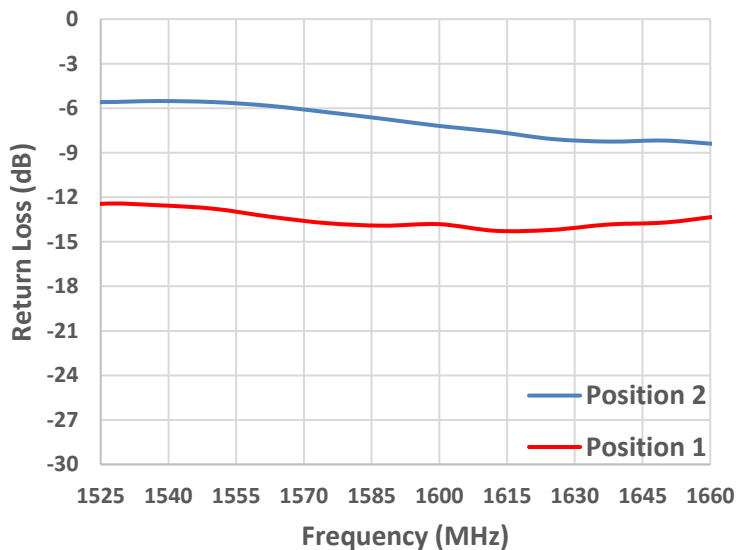
Return Loss (Band 255: 1525 - 1660 MHz)
