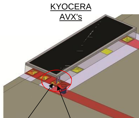
Shorting pin and feed pin are shared in KYOCERA AVX's ceramic antennas
