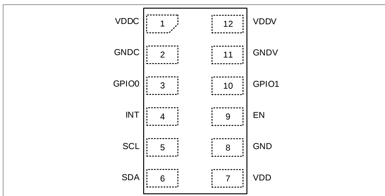
Figure 2: Pin locations top through view (not to scale)
