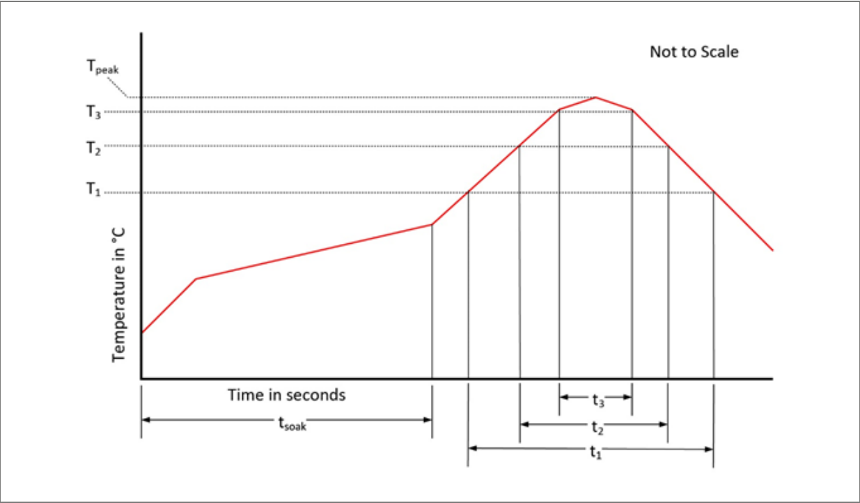
Figure 18: Solder reflow profile graph
