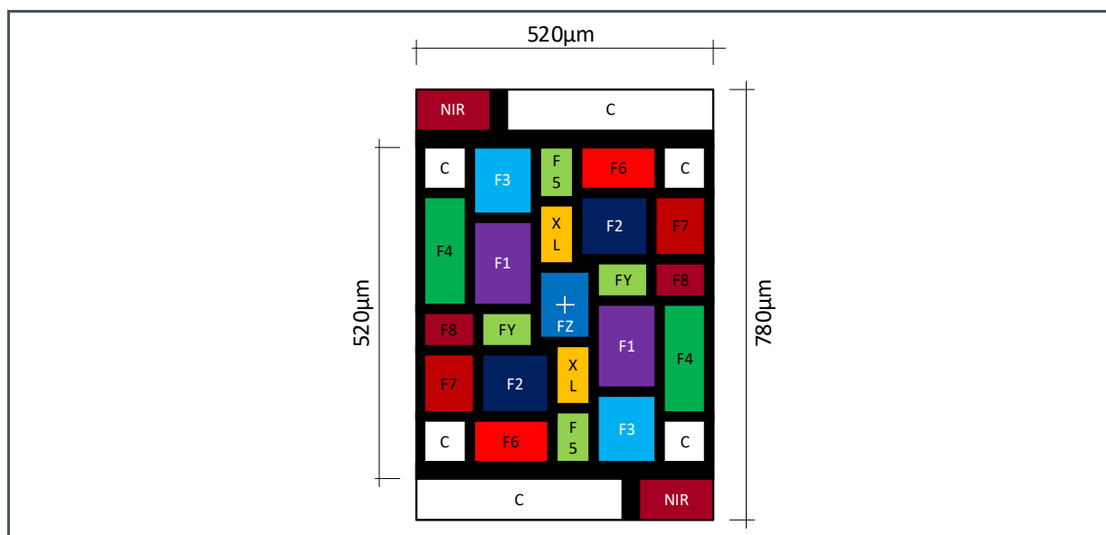
Figure 14: Sensor Array
