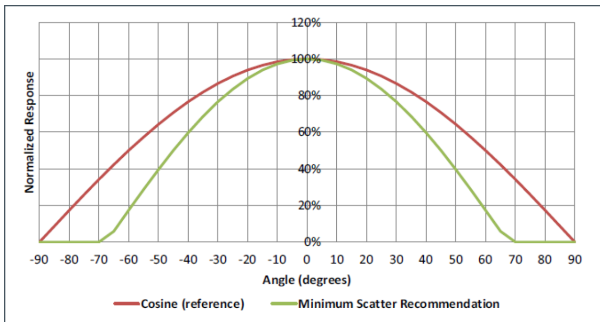
Figure 60: Diffuser Characteristics
