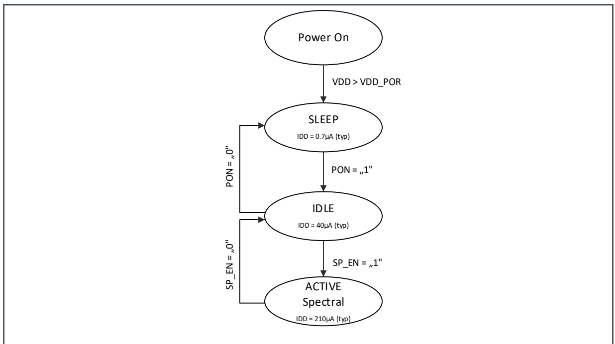
Figure 12: Simplified State Diagram
