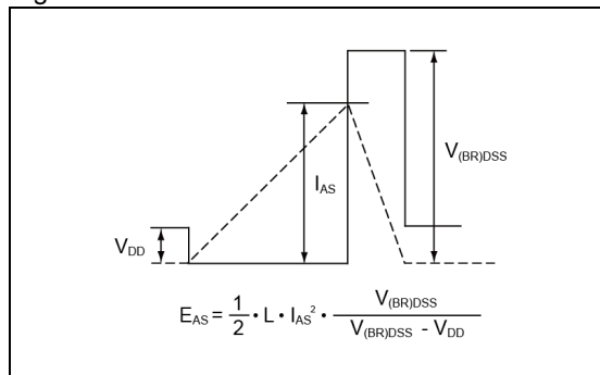
Fig.6-2 Avalanche Waveform
