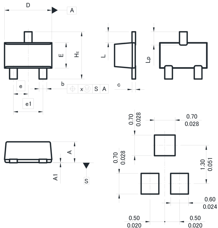
Soldering footprint Unit: ( mm / inches )
