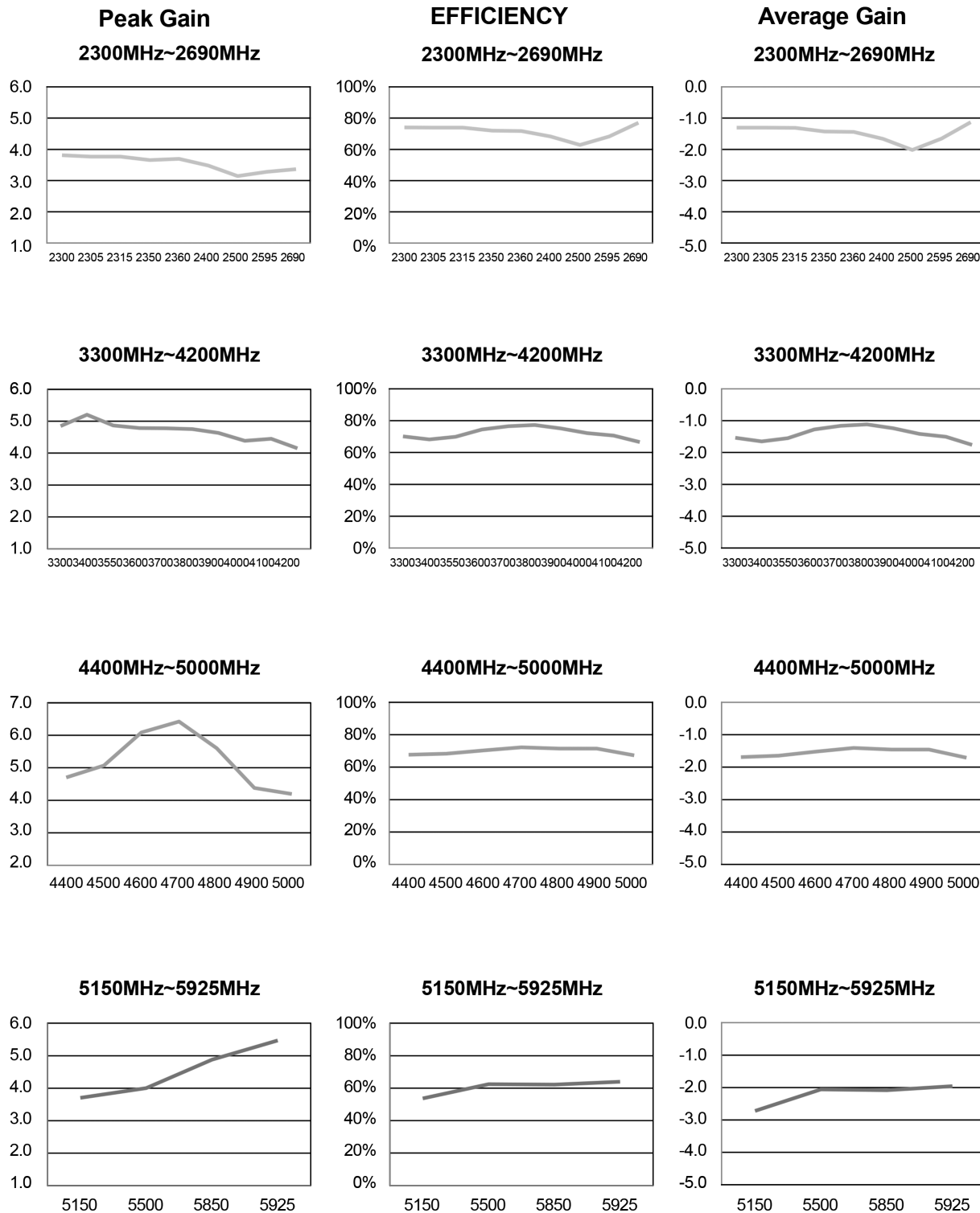
Gain Table (with 185mm × 165mm Metal housing)
