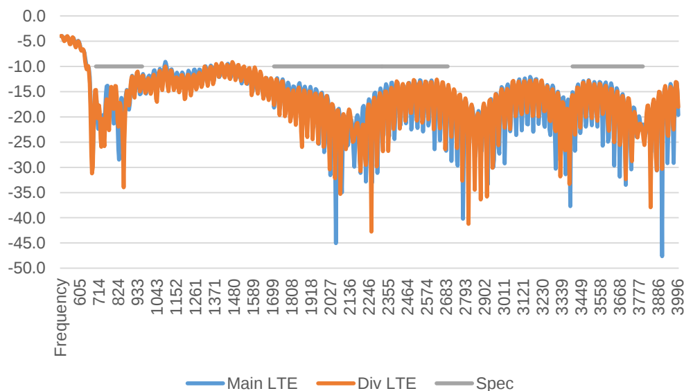
Return Loss
