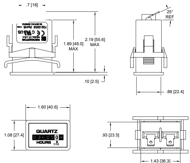
Flush-Rectangular
