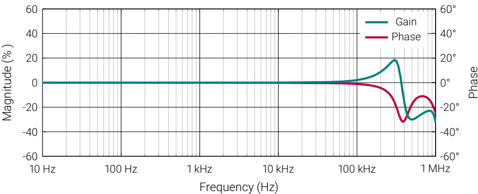
Figure 5: Frequency characteristics
