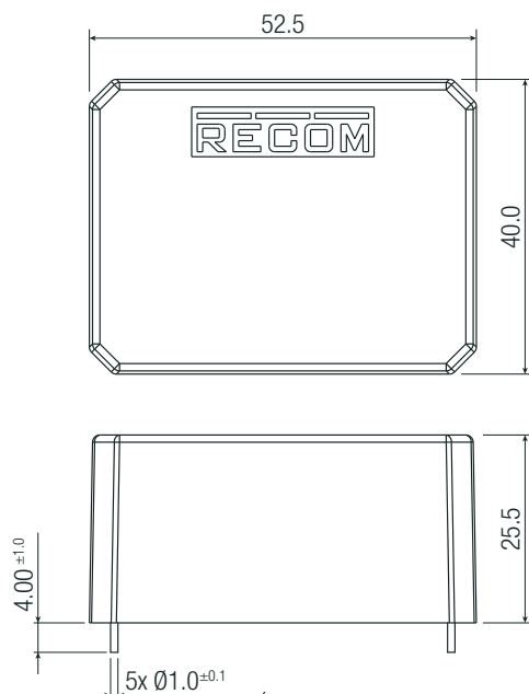
Dimension Drawing standard THT version (mm)
