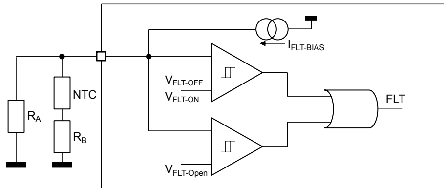
Figure 18. Fault pin block diagram
