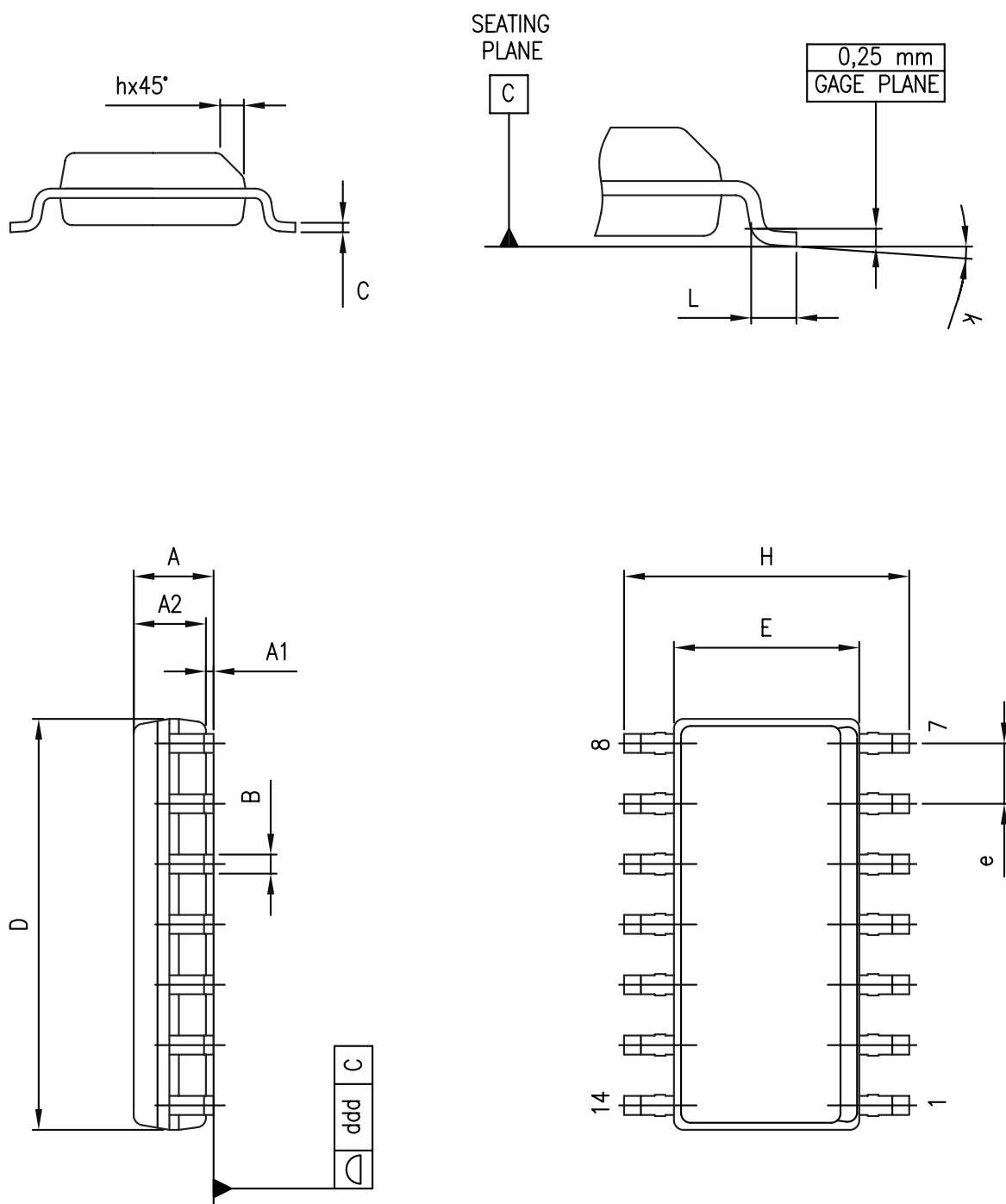
Figure 19. Package dimensions
