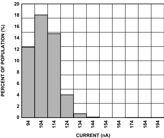
Figure 18. Standby Mode Current Consumption at 25°C, V_S = 2.5\text{ V}
