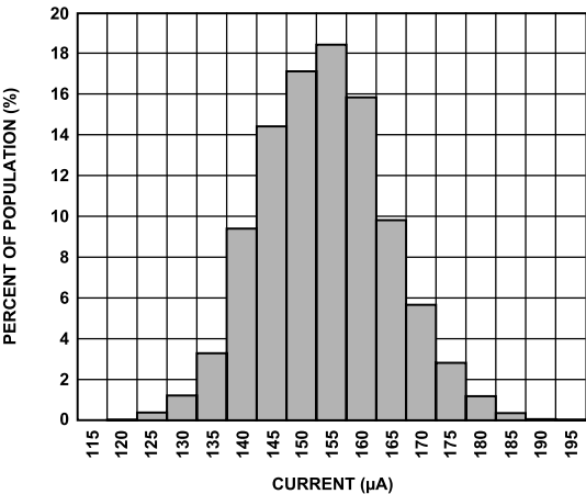
Figure 17. Measurement Mode Current Consumption at 25°C, V_S = 2.5\text{ V}
