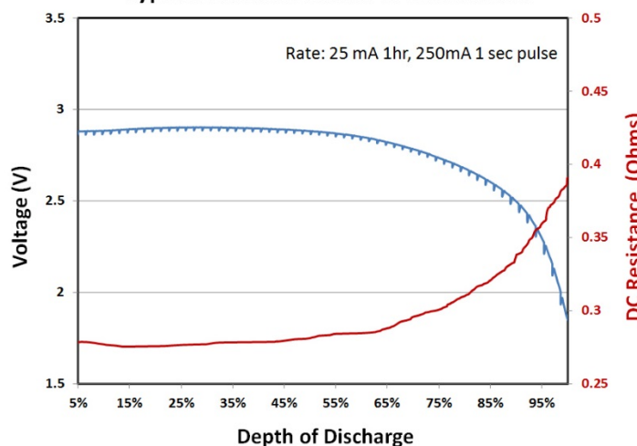
Typical Duracell DL123A Performance
