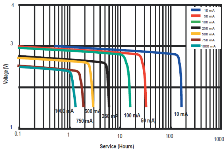
Continuous Discharge RT to 1.55 Volts
