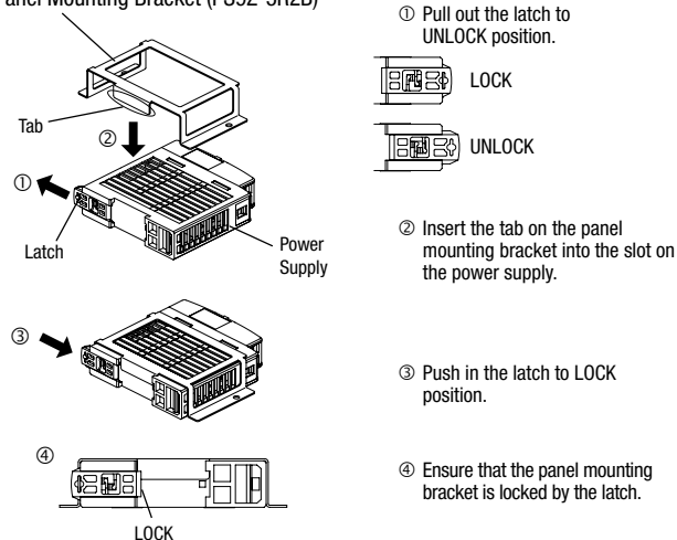
Panel Mounting Bracket (PS9Z-5R2B)
