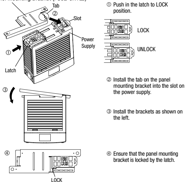
Panel Mounting Bracket (PS9Z-5R1□)
