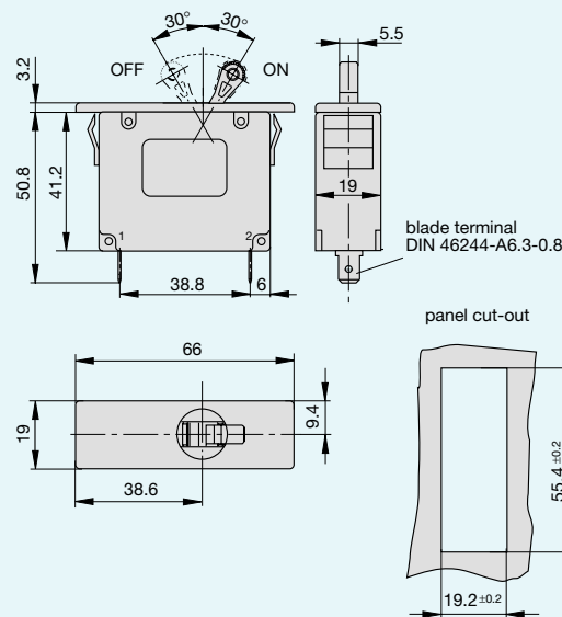
Mounting configuration 8340-F9..
