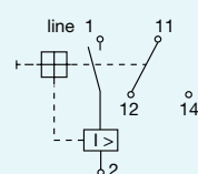
1 pole protected hydraulic-magnetic
