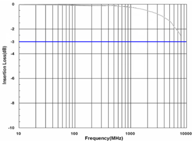
Insertion Loss
