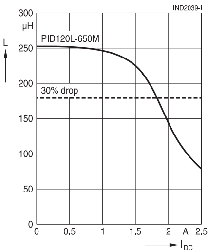
PID120L-650M
