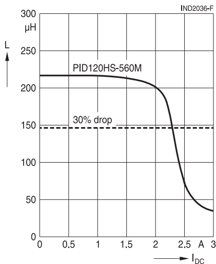
PID120HS-560M
