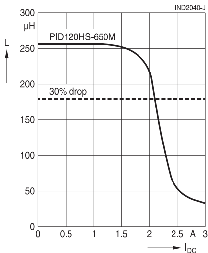
PID120HS-650M
