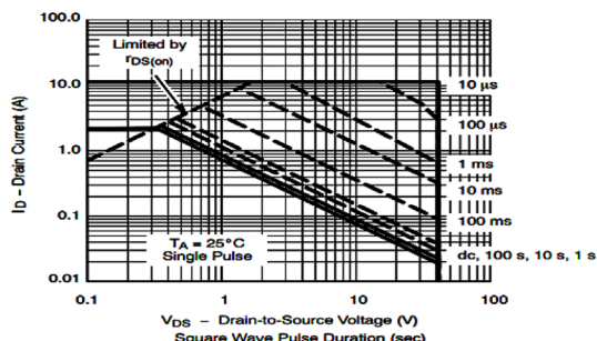
Fig 11: Safe Operating Area, Junction-to-Case
