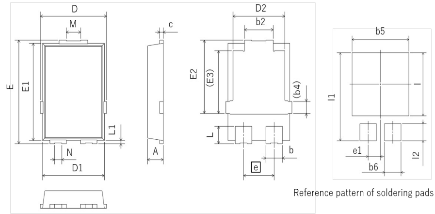
TO-277A
