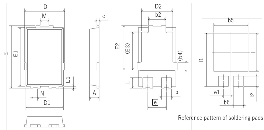
TO-277A
