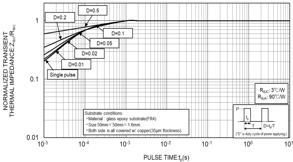
NORMALIZED TRANSIENT THERMAL IMPEDANCE FROM JUNCTION TO CASE (PER DEVICE)
