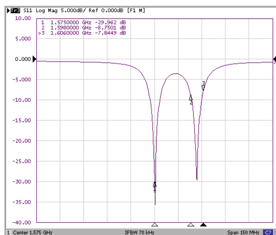
(Return Loss)
