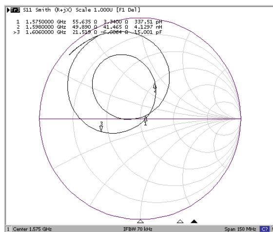
(Impedance)
